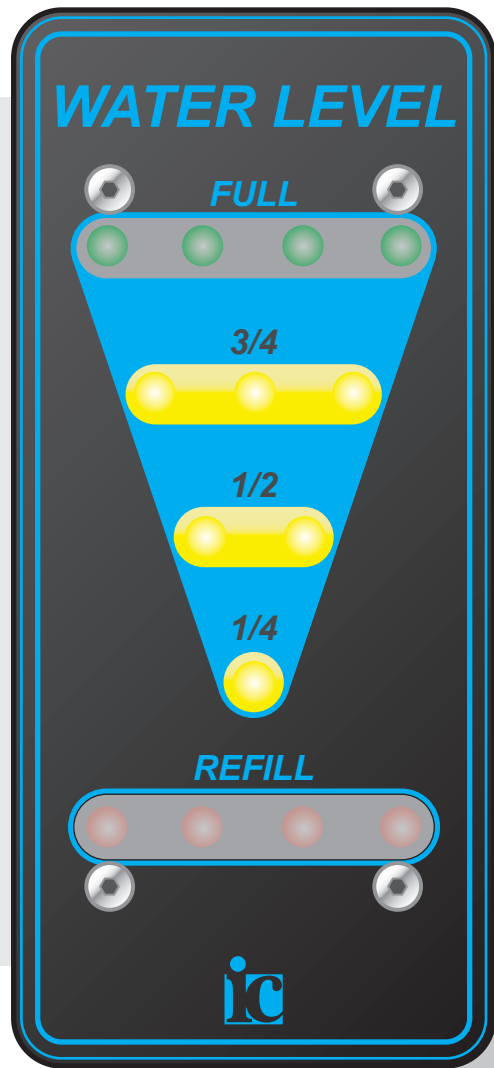
14-LED Master Water Display P/N 3030068
