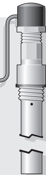
Thread-Mount Tank Sender P/N 3030214-01-XX
