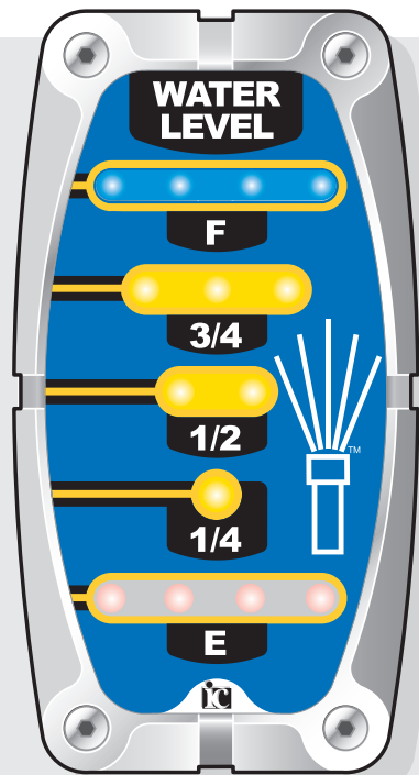
14-LED Master Water Display P/N 3030086
