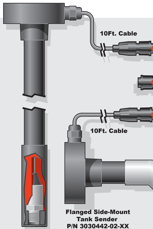
Flanged Top-Mount Tank Sender P/N 3030213-02-XX
