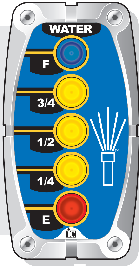
5-Light Master Water Display P/N 3030087
